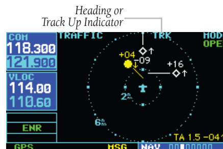
Figure 12-5 Traffic Page
