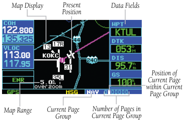
Figure 3-8 Map Page
