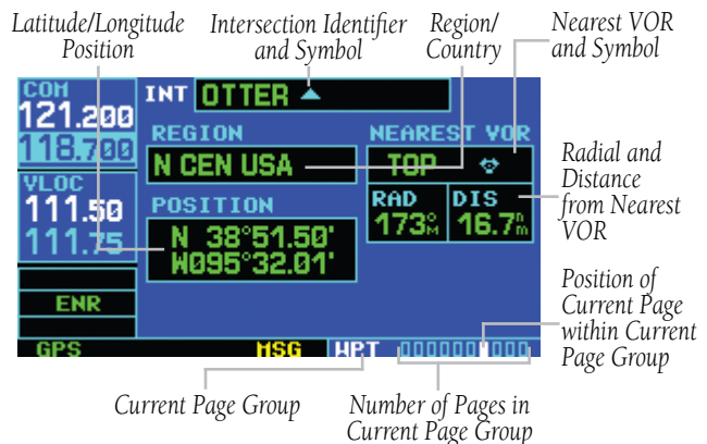
Figure 7-31 Intersection Page
